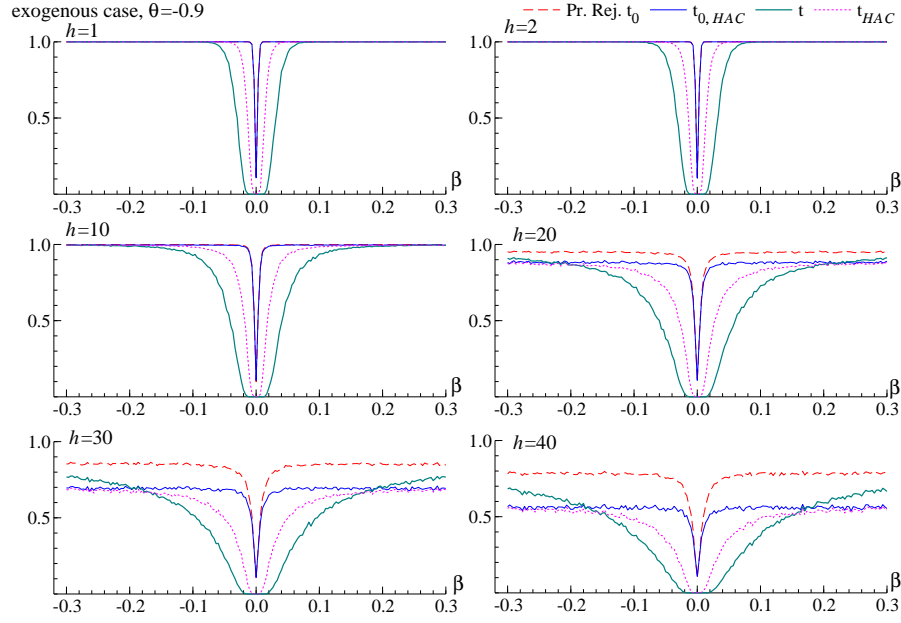
Figure 7: The figure reports the rejection probabilities of four test statistics ( t_0 , t_{0,HAC} , t and t_{HAC} ) for the null that \beta = 0 . The sample size is T = 250 observations, \theta = -0.9 and there is no endogeneity.
