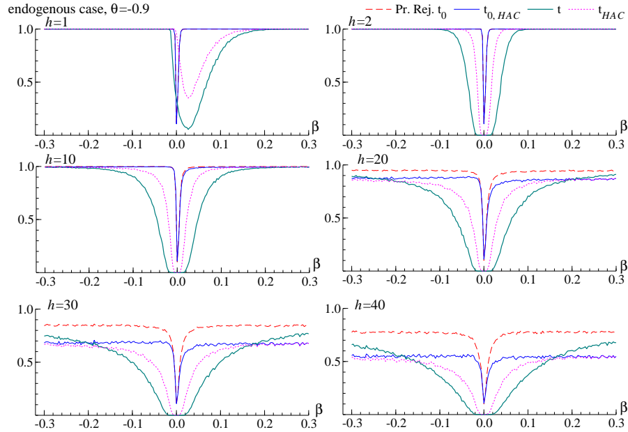
Figure 8: The figure reports the rejection probabilities of four test statistics ( t_0 , t_{0,HAC} , t and t_{HAC} ) for the null that \beta = 0 . The sample size is T = 250 observations, \theta = -0.9 and there is contemporaneous endogeneity: \text{Corr}(\varepsilon_t, \epsilon_t) = 1/\sqrt{2} .
